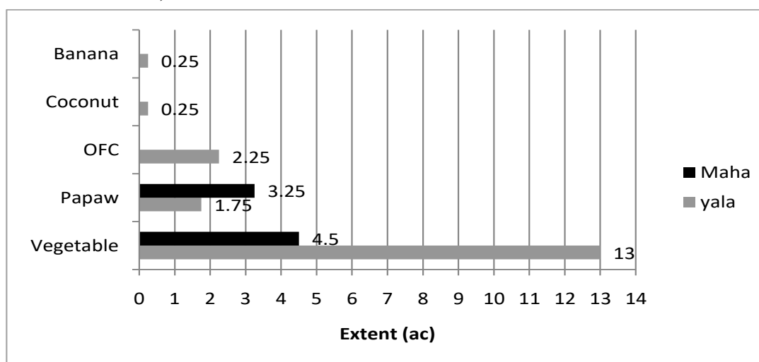
Figure 5.3: Total Extent Cultivated by Sample Farmers Using Drip System (In acres)
